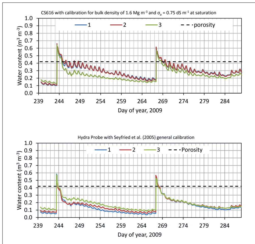
Fig. 7. CS616 water contents from calibration for sandy clay loam with bulk electrical conductivity = 0.75 dS m -1 at saturation (top); and Hydra Probe water contents using Seyfried et al. (2005) general calibration (bottom). All were installed at the same depth in a uniformly wetted soil. This soil cannot become wetter than the 0.42 ft/ft water content marked with the dashed line because that is the porosity of the soil.
